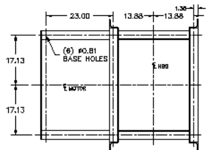
FOUNDATION PLAN - TOP VIEW
