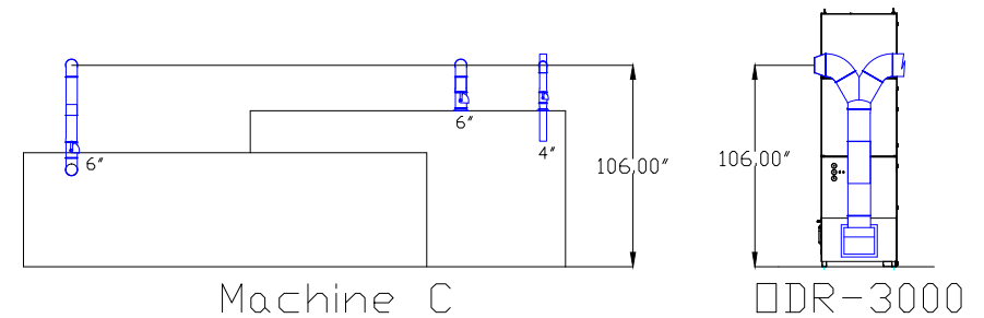
Elevation View
