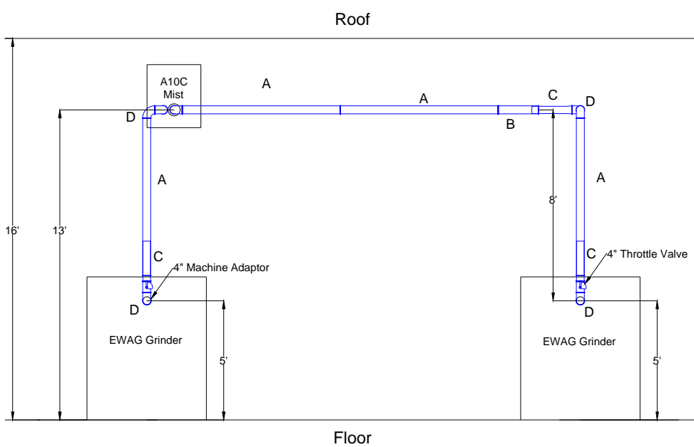
Elevation View
