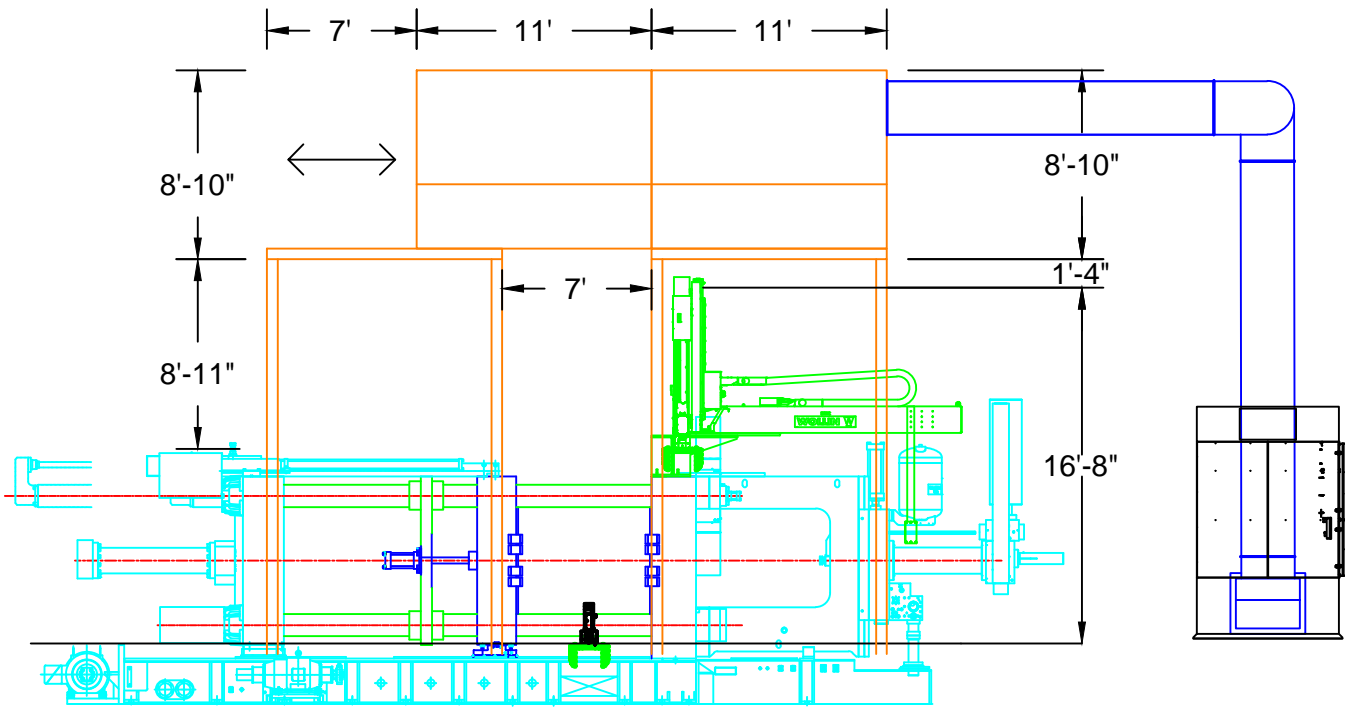
Side View
