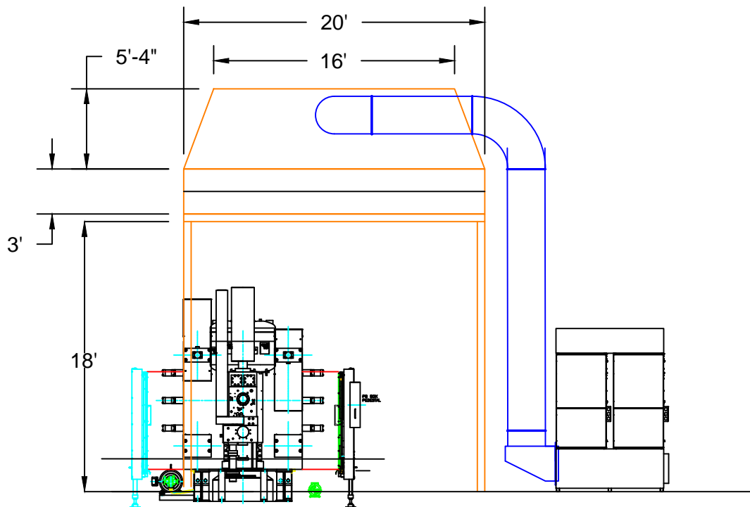
End View
