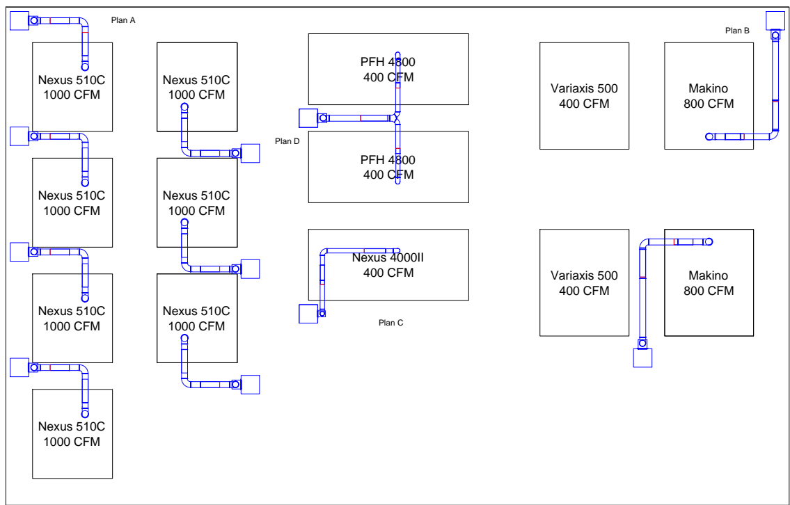
Plan View
