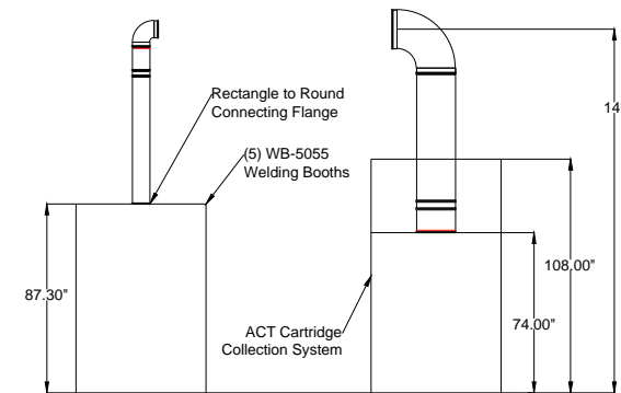
Elevation View
