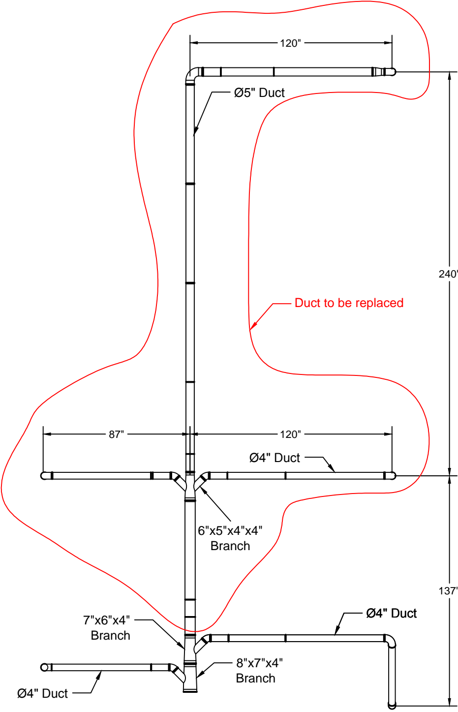
Elevation View
