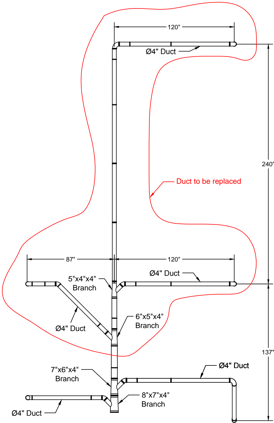
Elevation View
