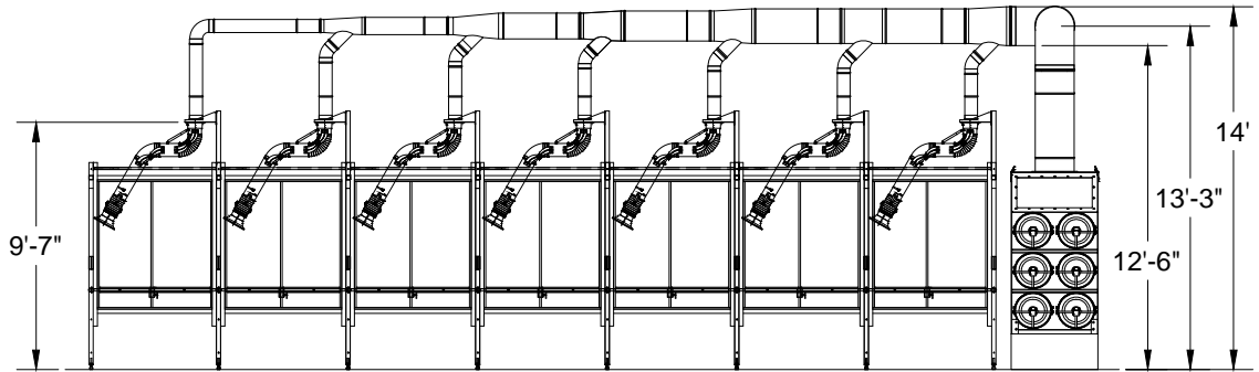
Elevation View
