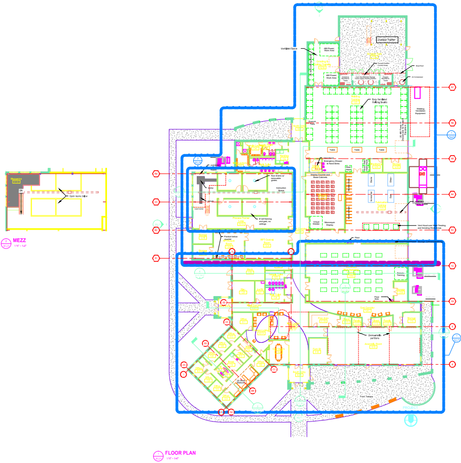
FLOOR PLAN 1/8" = 1'-0"
