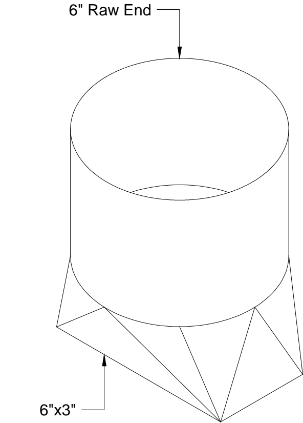
Isometric View
