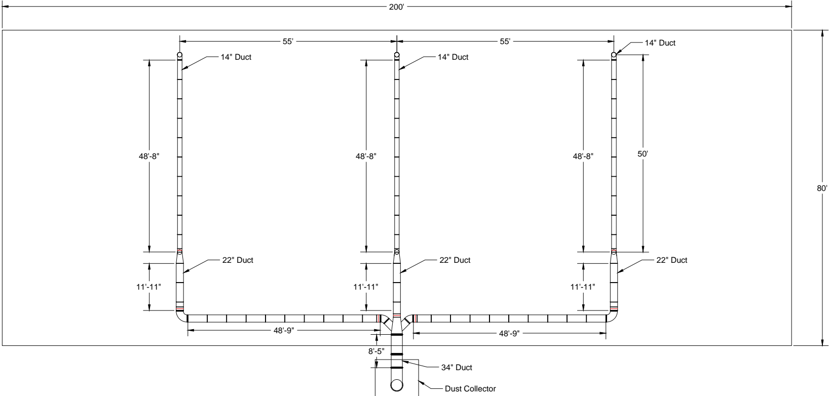
Plan View (Intake)
