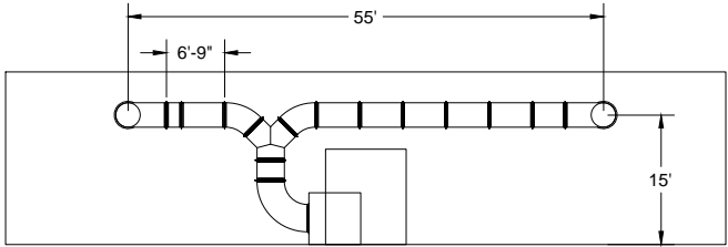
Front View (Return)
