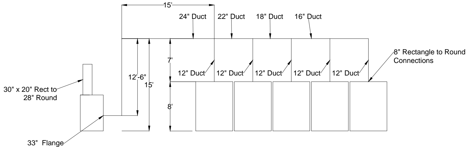
Elevation View
