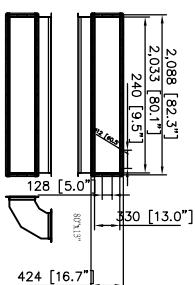
Flange TOP VIEW
