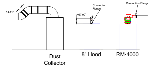
Elevation View
