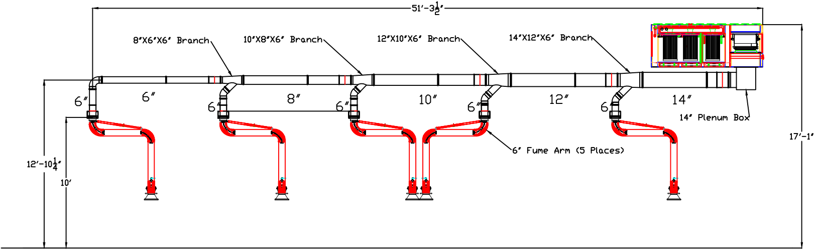
Elevation View
