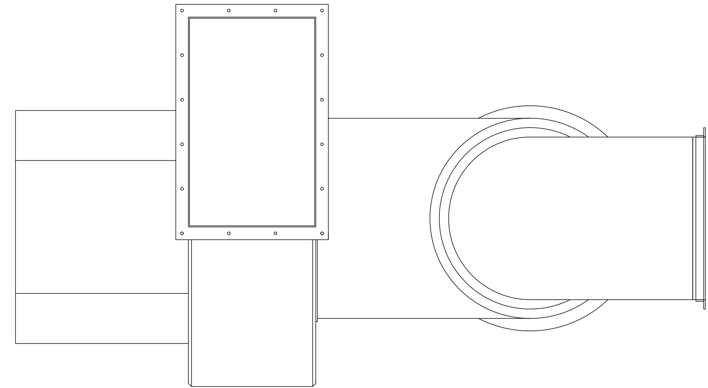
Plan View
