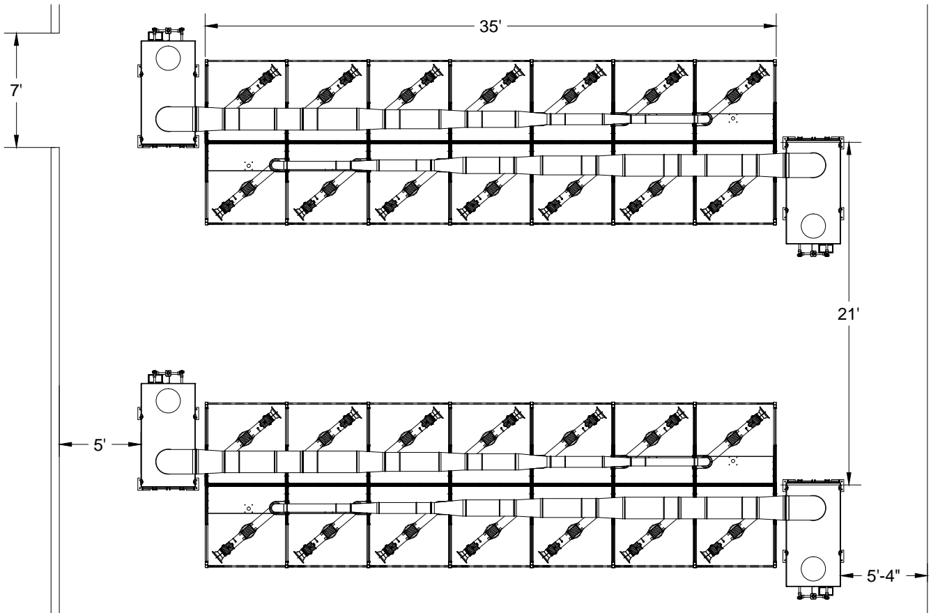
Plan View
