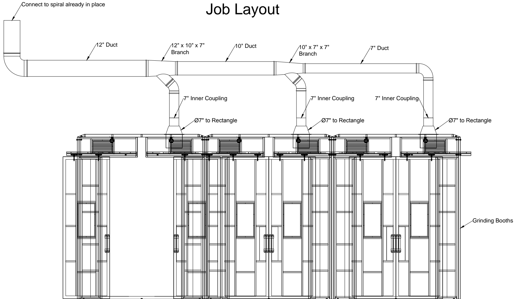
Plan View
