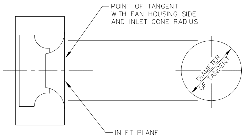
B. FREE INLET AREA PLANE -- FAN WITHOUT INLET COLLAR. WITHOUT INLET COLLAR.
