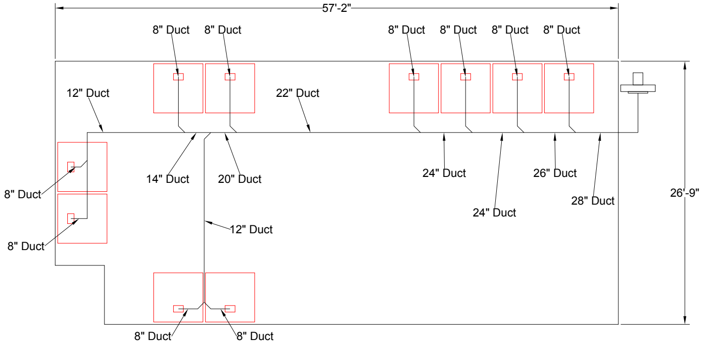
Plan View
