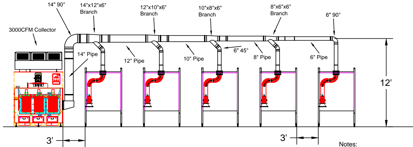
Elevation View
