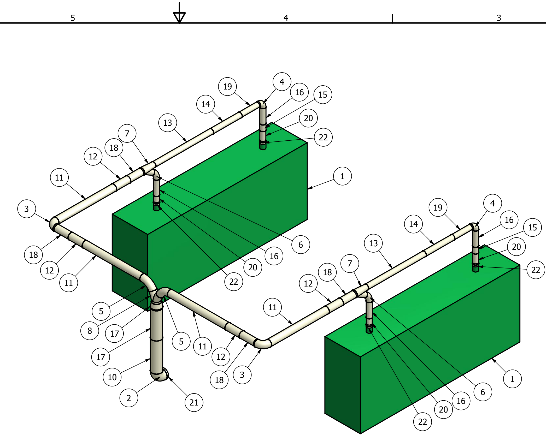
ISOMETRIC VIEW SCALE: 1/4"=1'-0"
