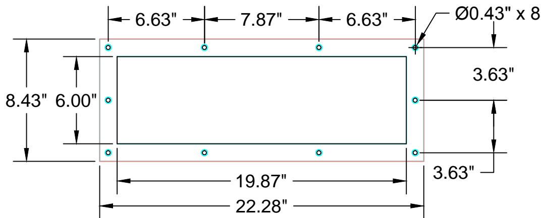
Flange View
