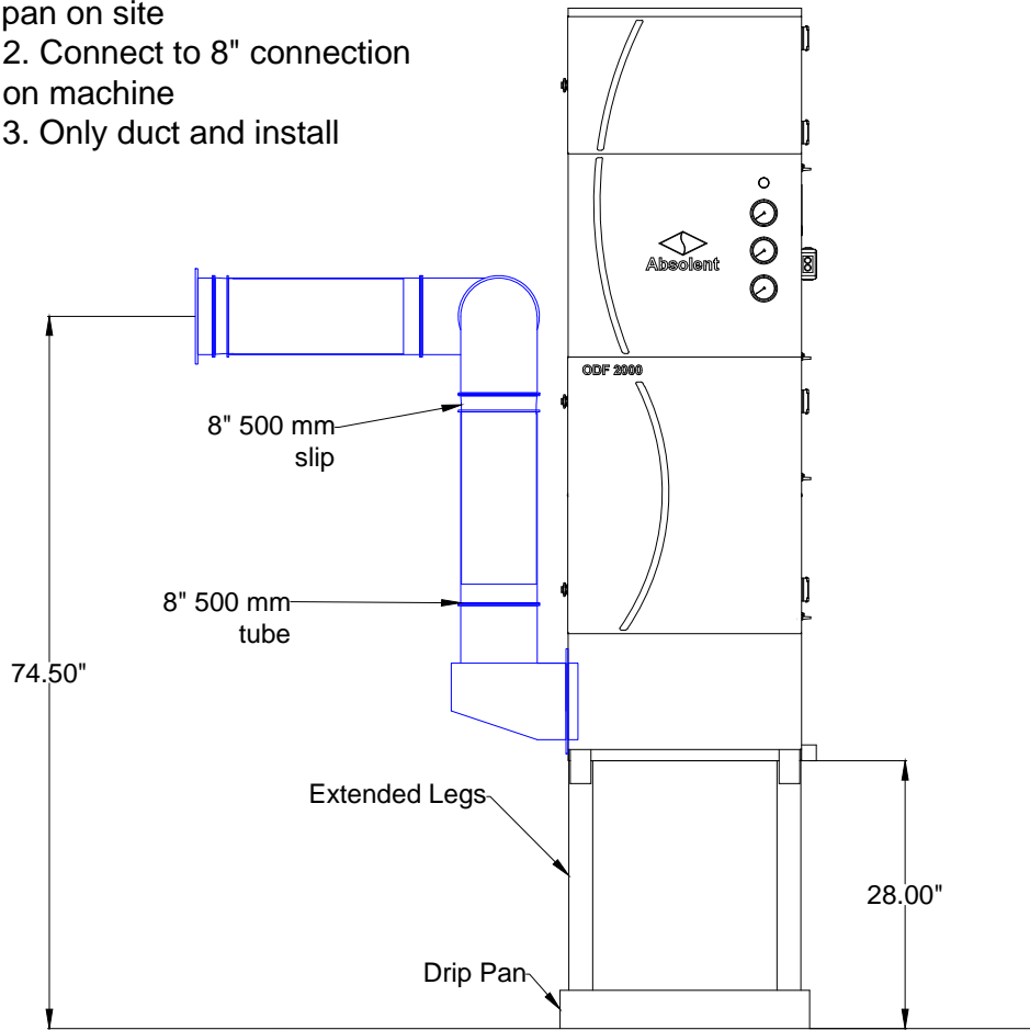
Elevation View
