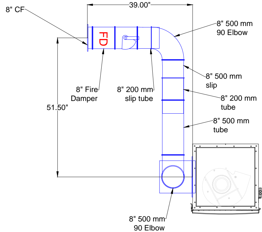
Plan View
