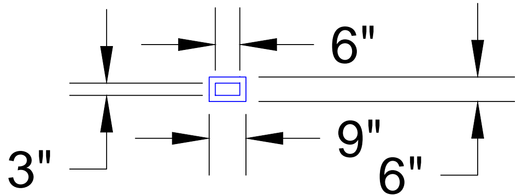
Flange View
