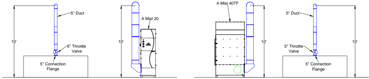
Elevation View
