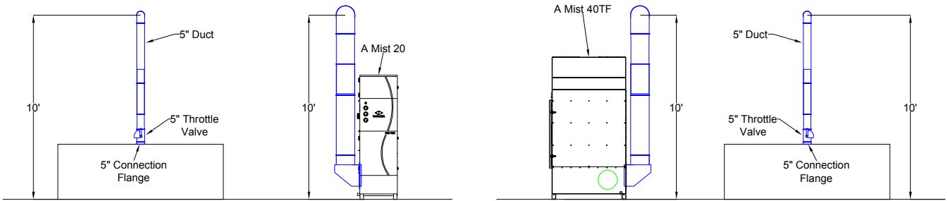
Elevation View
