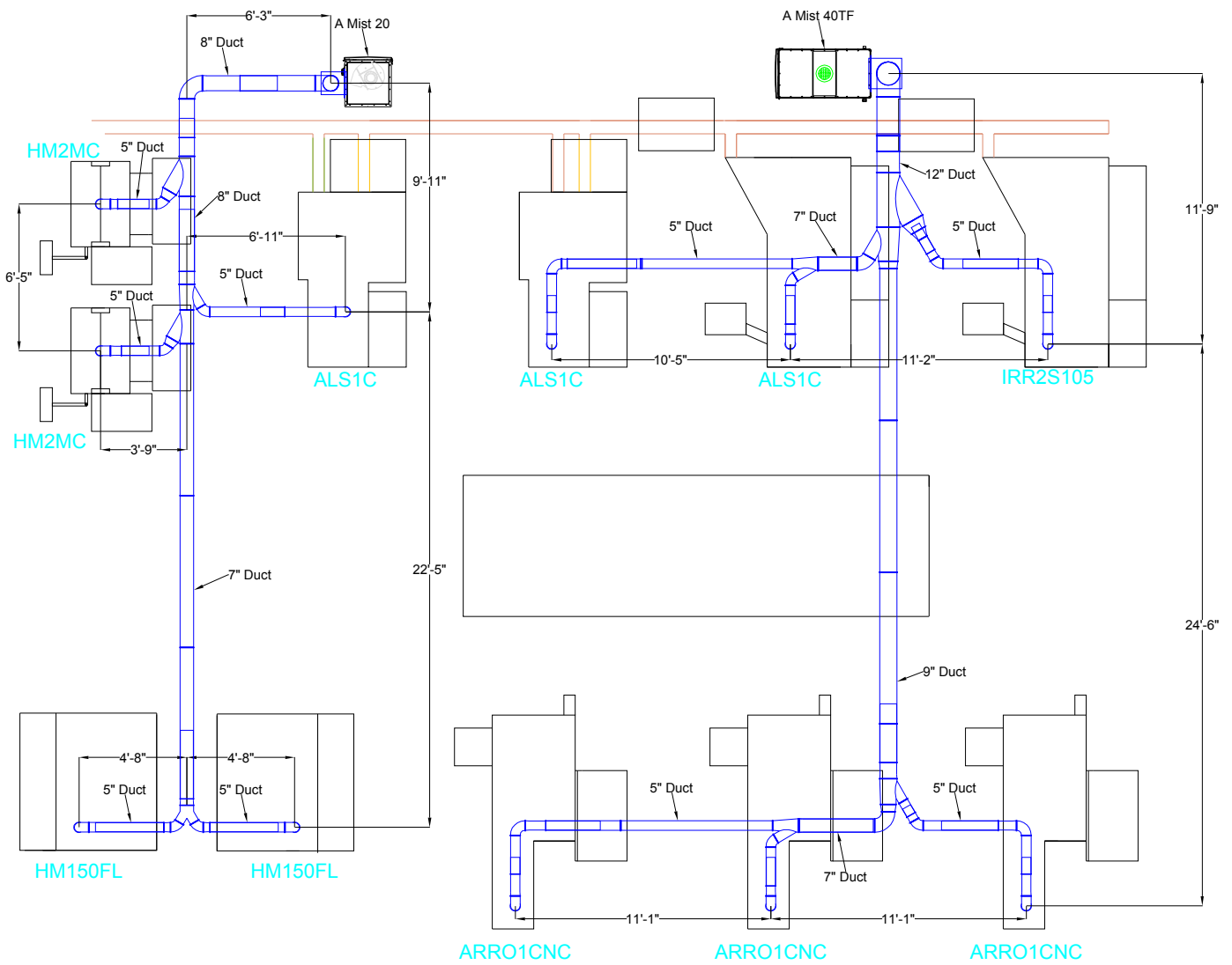
Plan View
