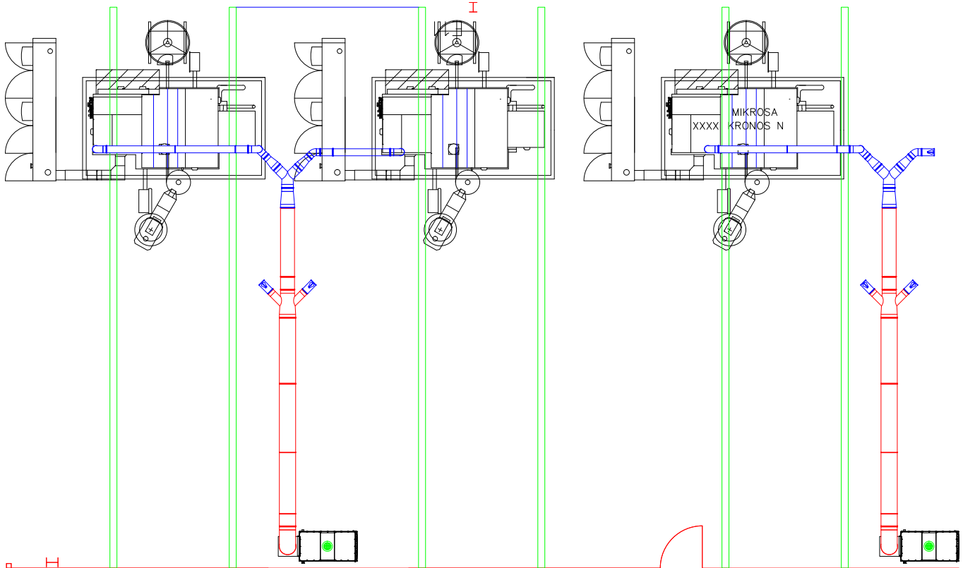
Plan View
