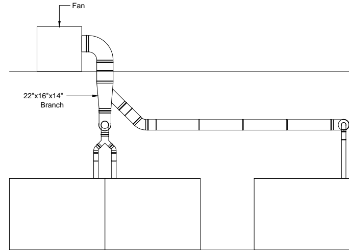
Elevation View C
