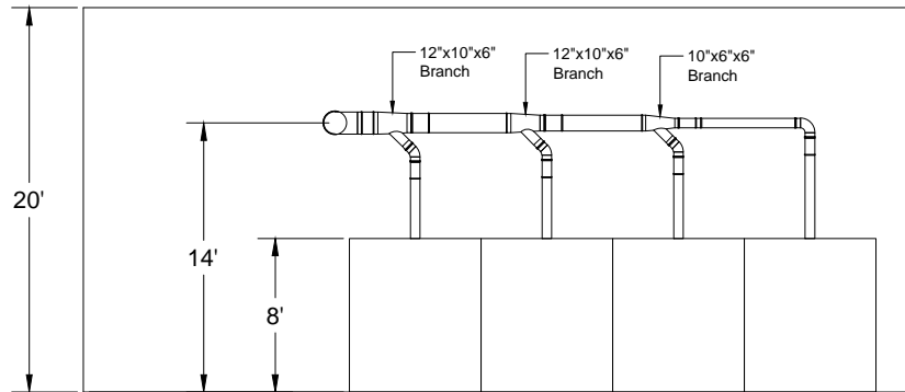
Elevation View A
