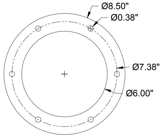
Flange View - Pipe
