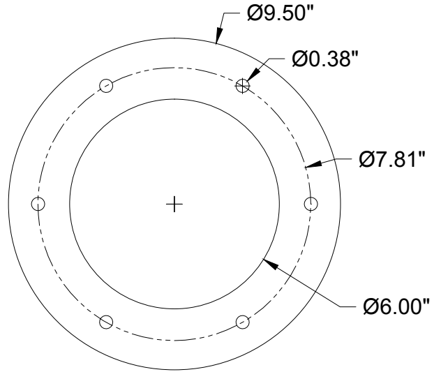
Flange View - Blower
