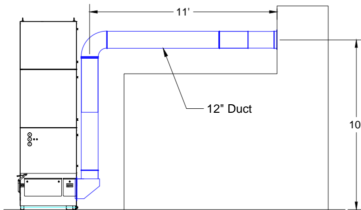
Elevation View
