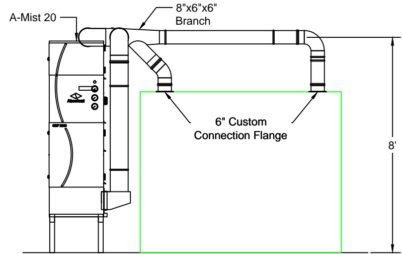
Elevation View
