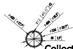
Collector Inlet
