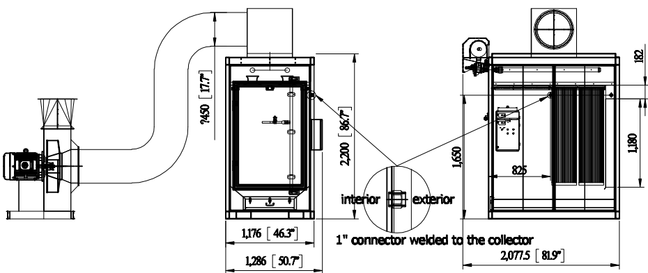
Blower
