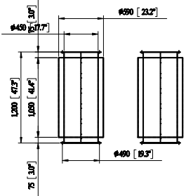
Silencer Outlet
