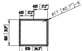
PLAN DETAIL
