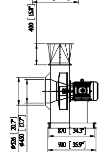
Blower
