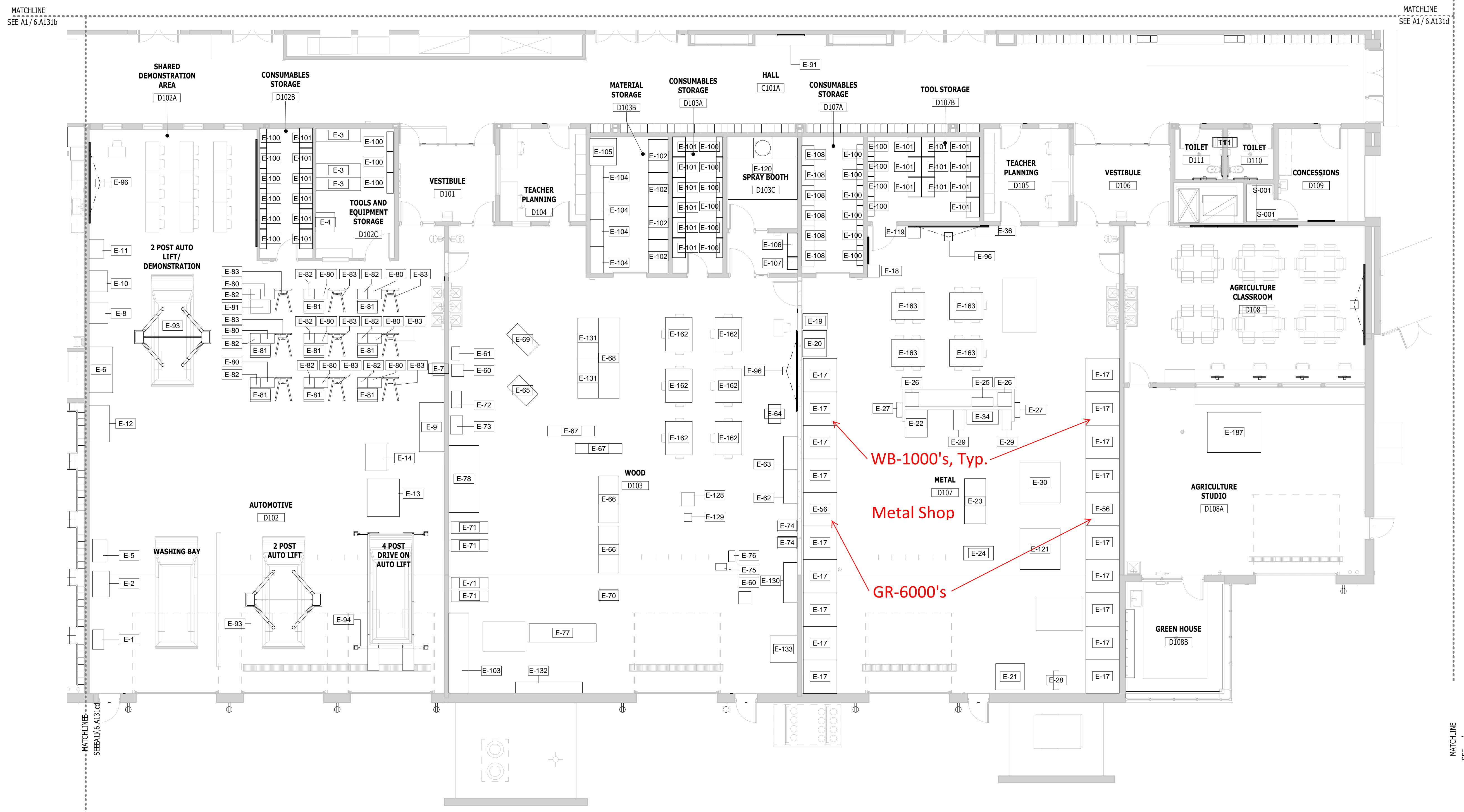
A1 LOWER LEVEL EQUIPMENT PLAN EA - AREA D 1/8" = 1'-0"
