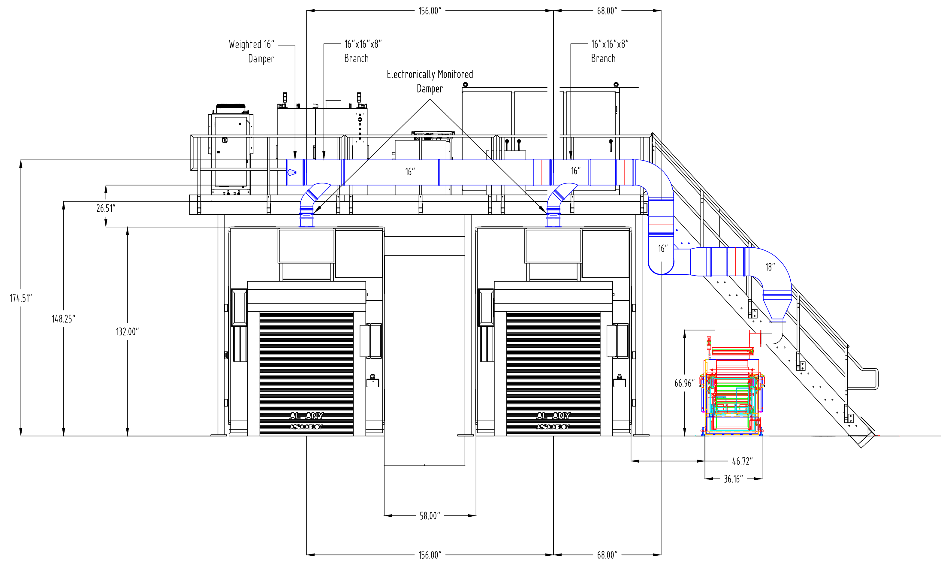
Elevation View
