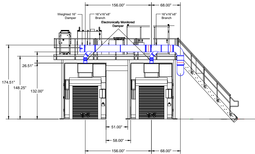
Elevation View
