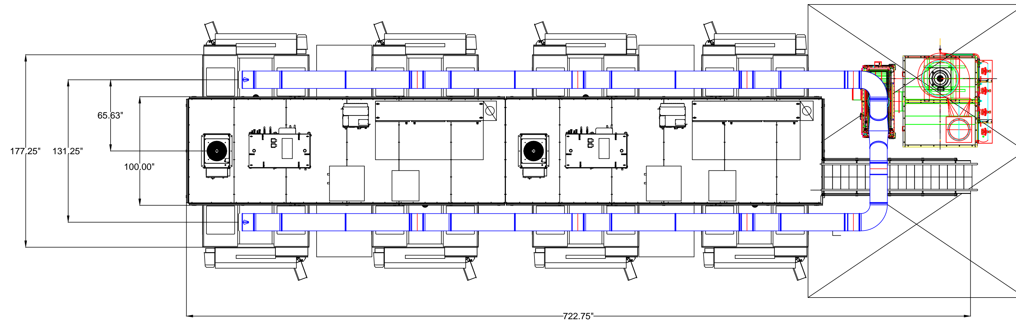
Plan View
