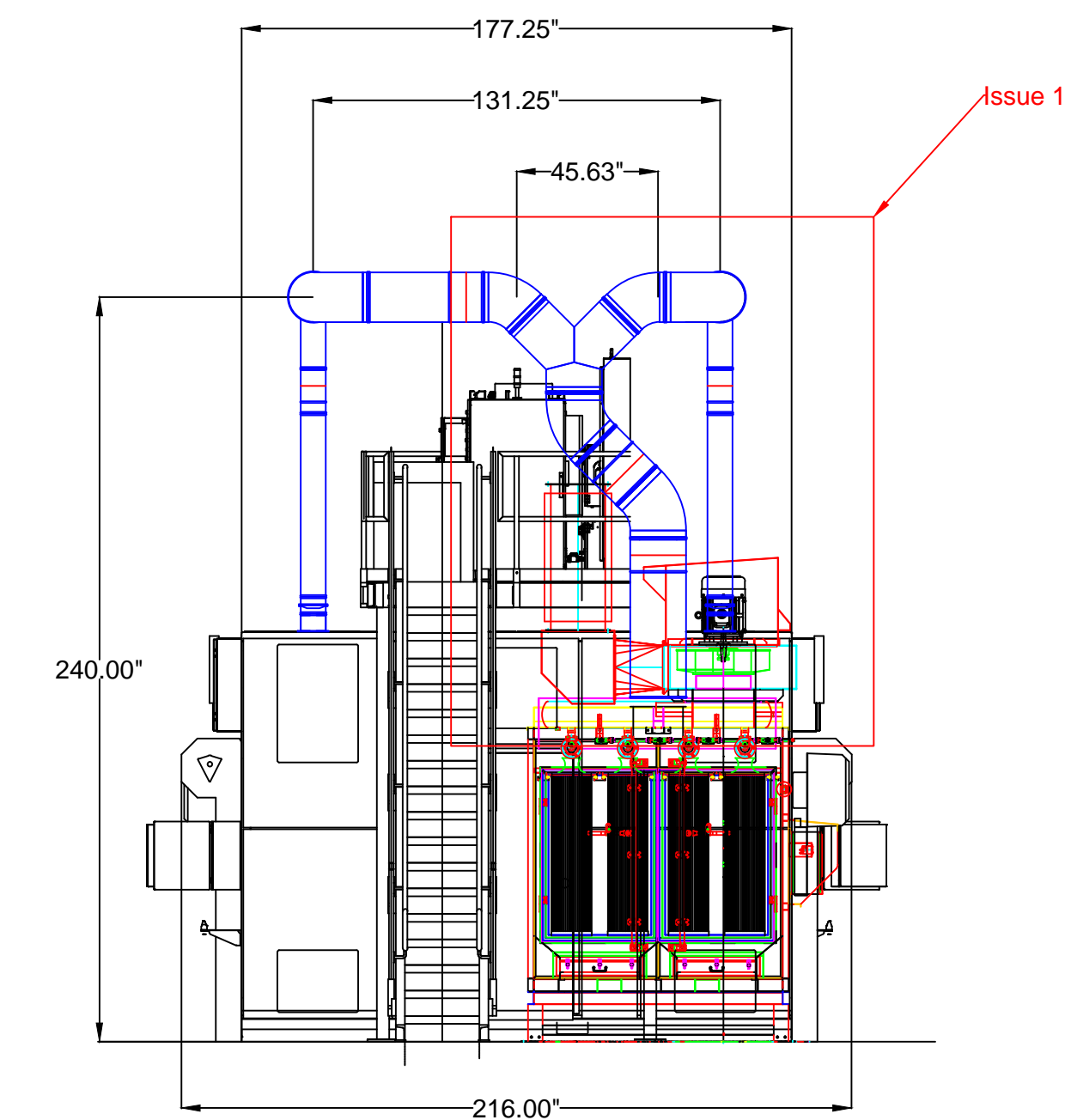
Side View
