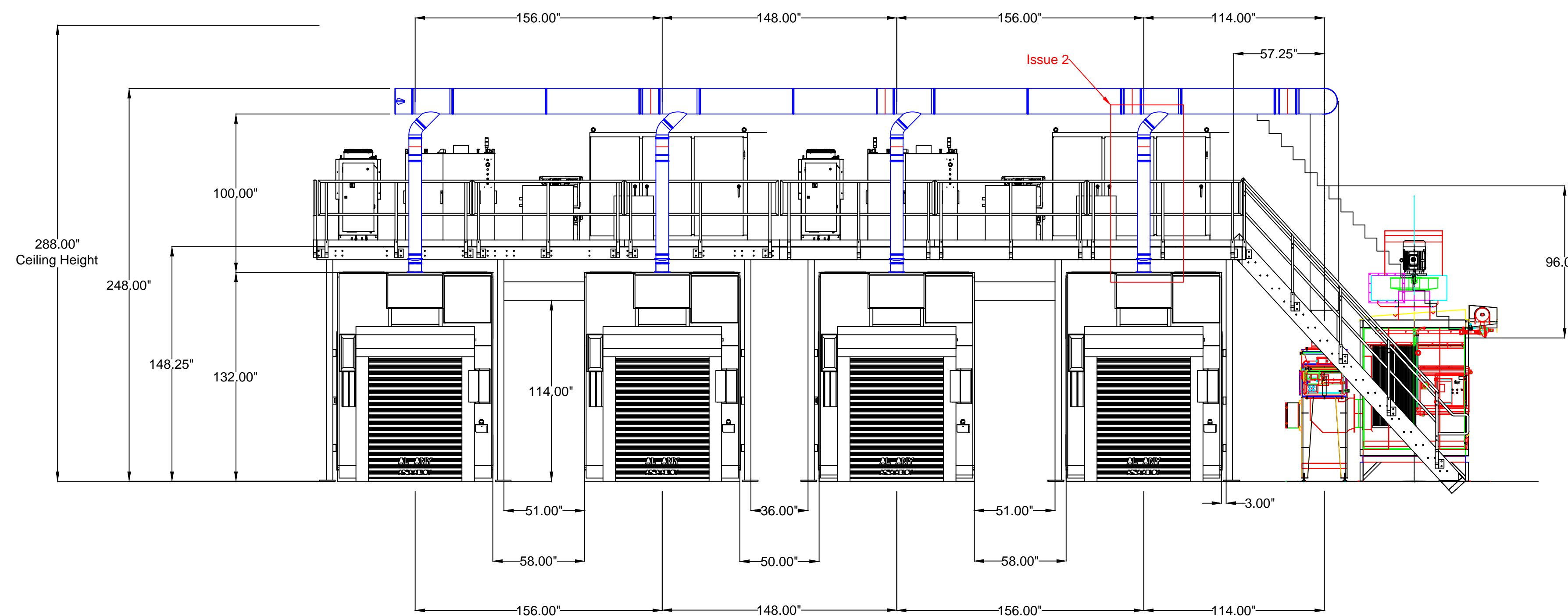
Elevation View
