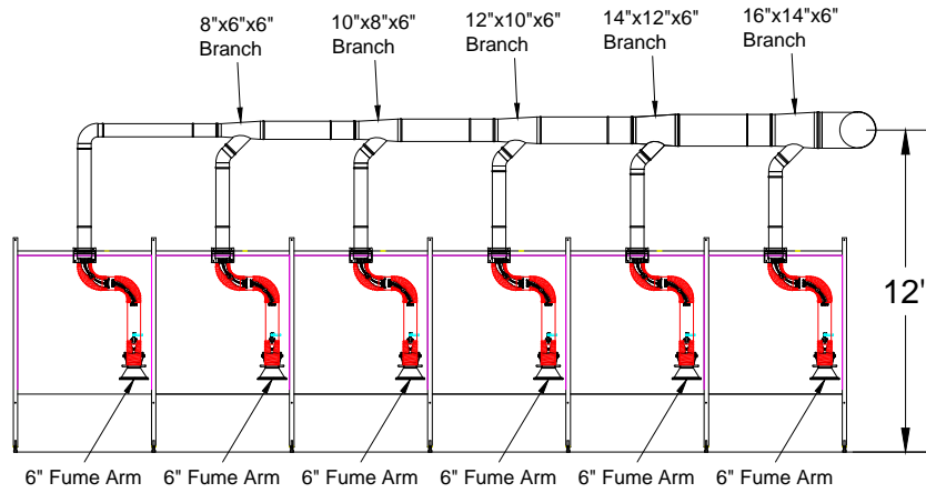
Elevation View
