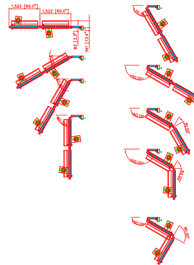
door operation
