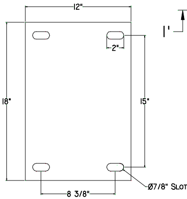
K-TRAC LIGHT DUTY FLOOR PLATE
