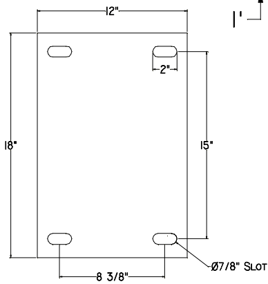
K-TRAC LIGHT DUTY FLOOR PLATE
