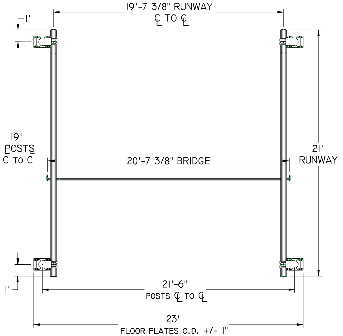
K-TRAC LIGHT DUTY FLOOR PLATE
