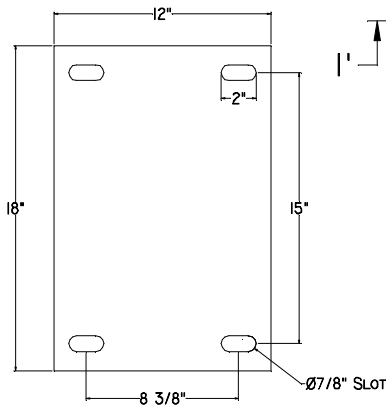
K-TRAC LIGHT DUTY FLOOR PLATE
