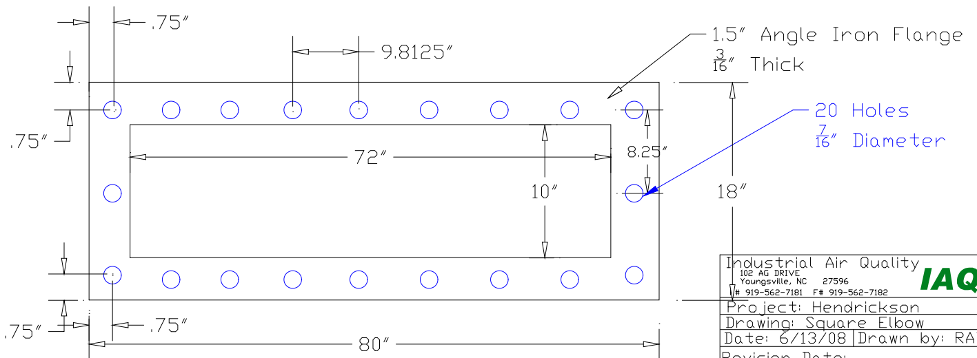
End View of Bolt Pattern
