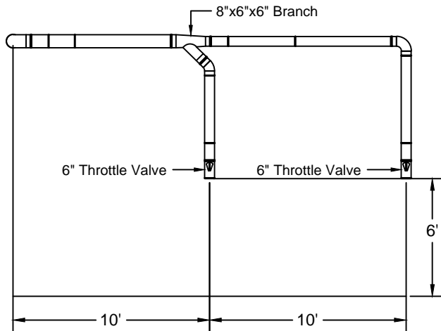
Elevation View
