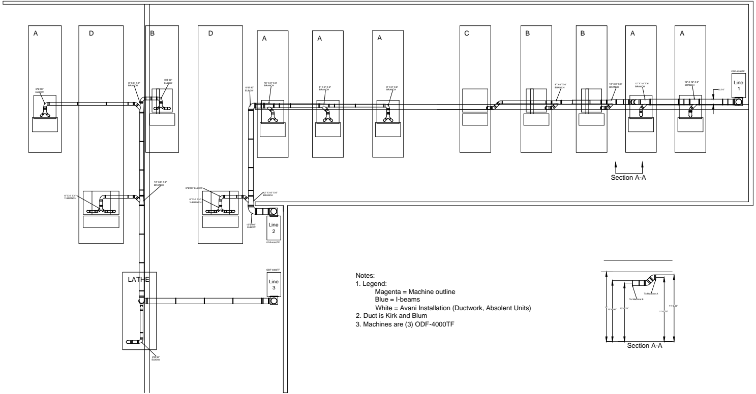
Plan View
