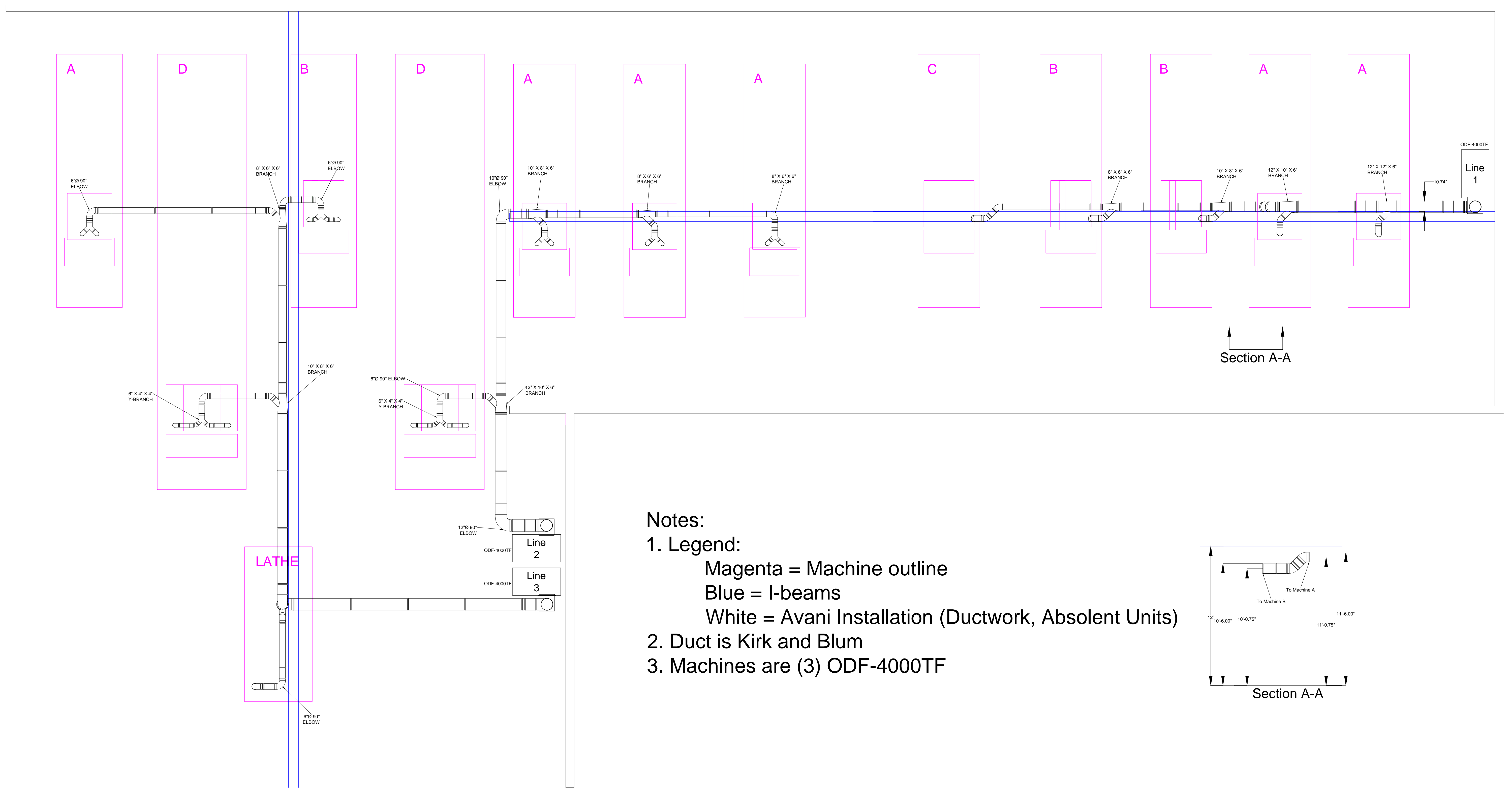
Plan View
