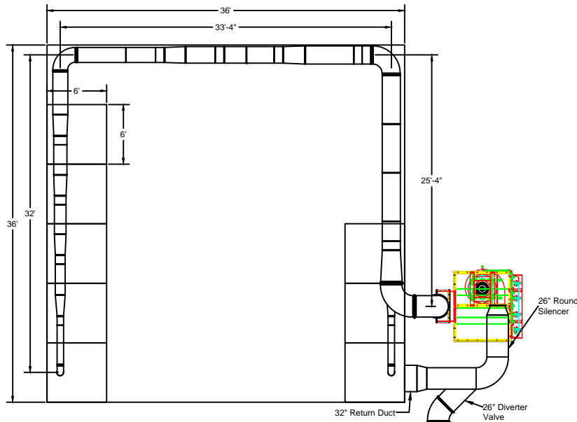
Overall Plan View
