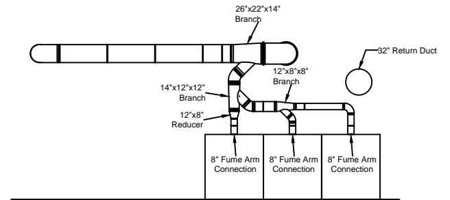
Right Side Elevation View
