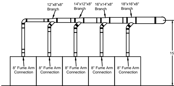
Left Side Elevation View
