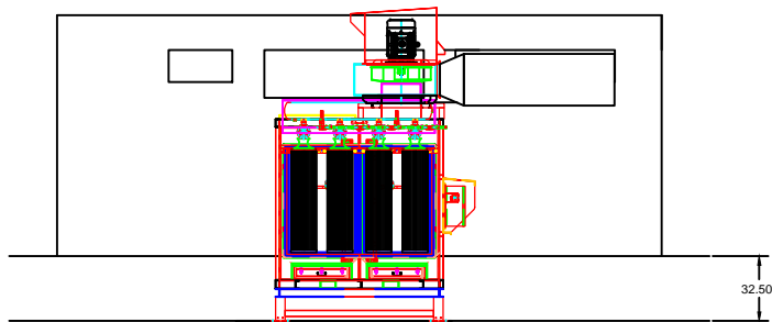
East Elevation Interior Front View
