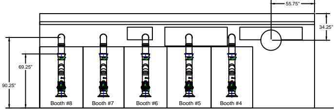
West Elevation Interior
