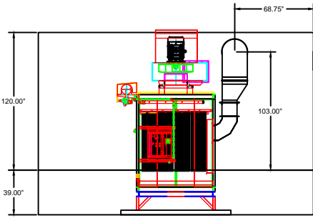
North Elevation Exterior Inlet Duct
