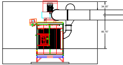
North Elevation Exterior Return Duct
